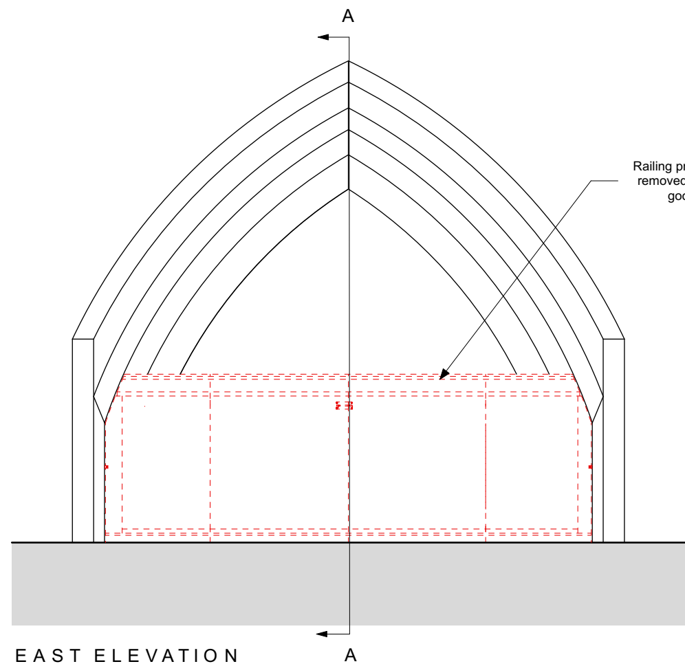
EAST ELEVATION
